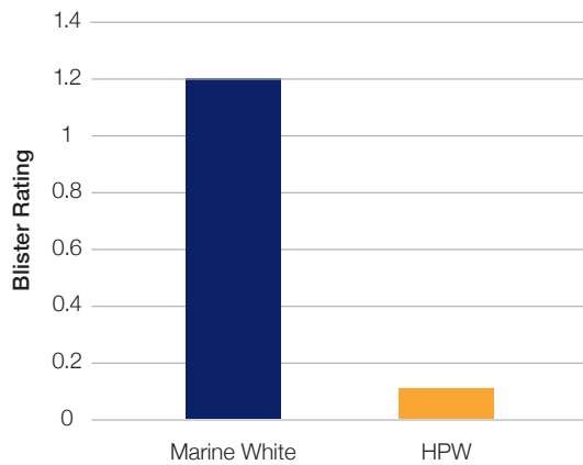
Blister Testing Marine White vs. HPW (150 °F at 1000 hours)
