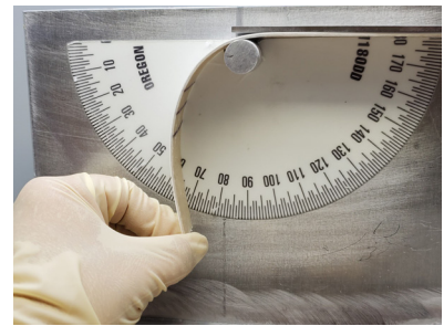
Mandrel bend test demonstrating HPW gelcoat's 50% increase in flexibility compared to other marine gelcoats.
