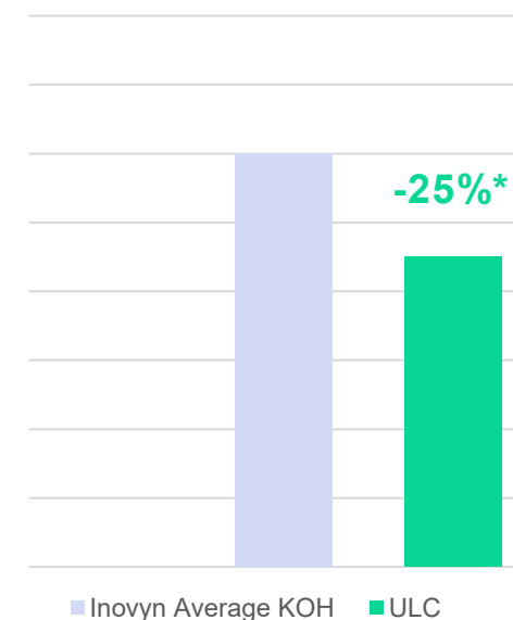
KOH GWP (in kg CO 2 eq/kg KOH)
