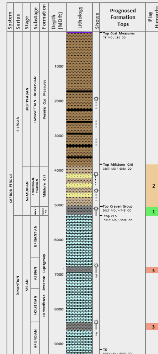
Anticipated Stratigraphic Succession
