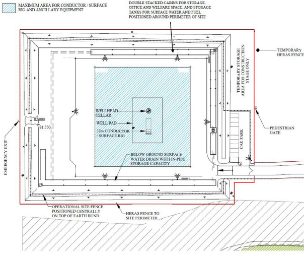
Plan shows end of Stage 1, just before the rig is brought to site.
