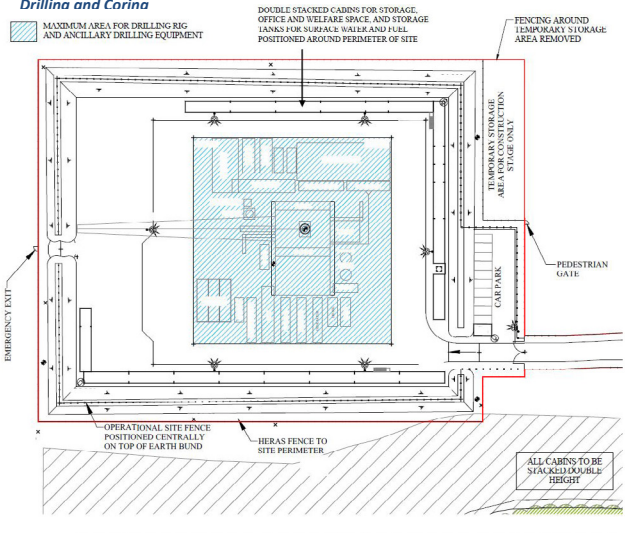
Plan shows site at the "peak" of activity, with the rig and all necessary drilling and coring equipment on site.
