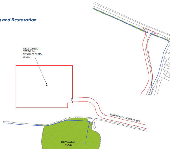
Plan shows site after completion of decommissioning and restoration. Decommissioning of the Stage 3 well would require a workover rig (<32 m) and associated equipment as shown in Stage 2. This would be temporary for a period of approximately 2 weeks, with removal of site equipment taking an additional 2 weeks, followed by a 3 week restoration period.
