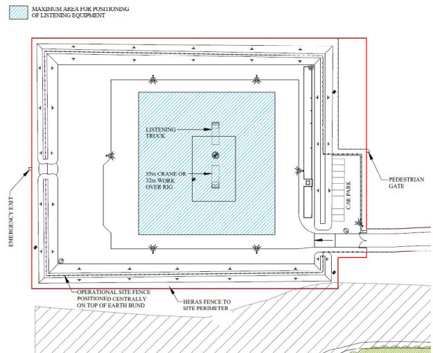
Plan shows site during listening operations with a listening truck and either a crane or a workover rig on site.
